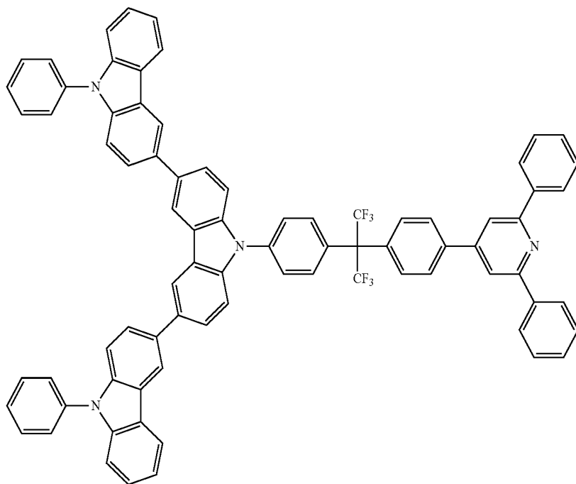
Compound 47
