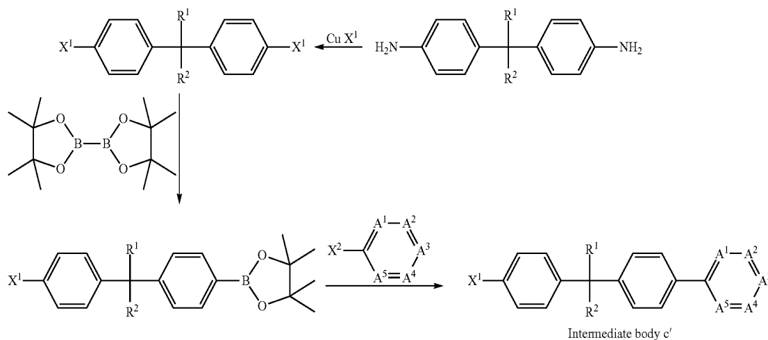
(Reaction formula 1)
