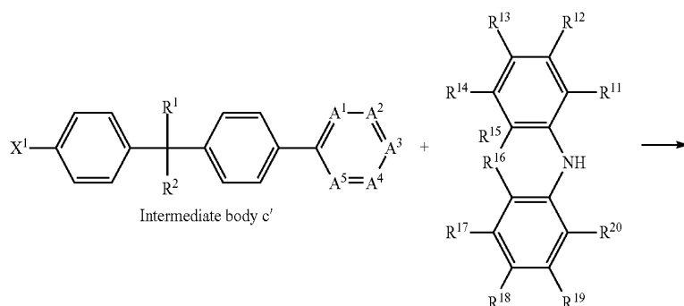
(Reaction formula 1)
