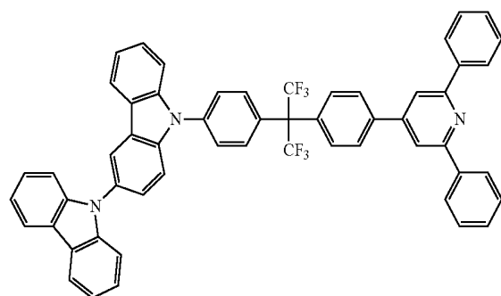
Compound 44
