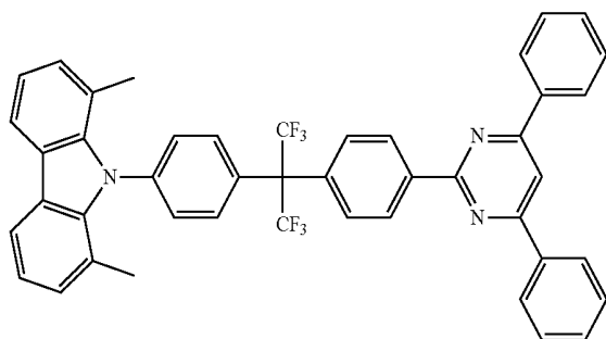
Compound 17
