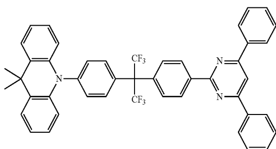
Compound 13
